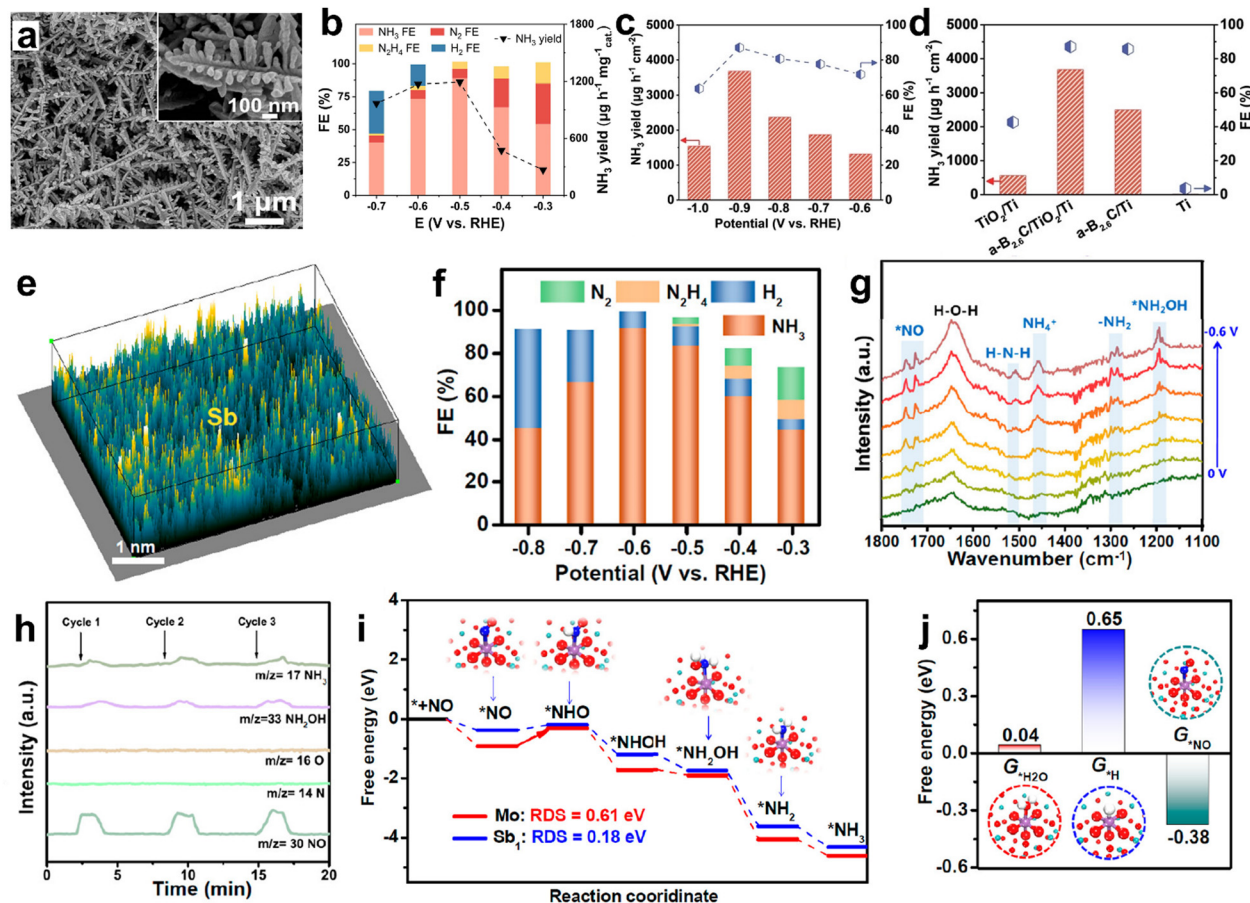
Fig. 9 (a) SEM image (inset: high-magnification image) of Bi NDs, (b) FEs of the major reductive products and NH 3 yields for Bi NDs/CP at each given potential. Reproduced with permission from ref. 111 copyright 2022, Elsevier. (c) FEs and NH 3 yields of a-B 2.6 C@TiO 2 /Ti at different potentials, (d) performance comparison. Reproduced with permission from ref. 113 copyright 2022, Wiley-VCH. (e) 3D atom image of p-block Sb single atoms confined in amorphous MoO 3 (Sb/a-MoO 3 ), (f) FEs of different products at various potentials, (g) potential-dependent in situ FTIR spectrum of Sb/a-MoO 3 from 0 to -0.6 V, (h) online DEMS spectrum of Sb/a-MoO 3 during the NORR electrolysis at -0.6 V, (i) free energy diagrams of alternating-N pathways on a-MoO 3 and Sb/a-MoO 3 , and (j) binding free energies of *H 2 O, *H, and *NO on Sb/a-MoO 3 . Reproduced with permission from ref. 115 copyright 2023, ACS.
