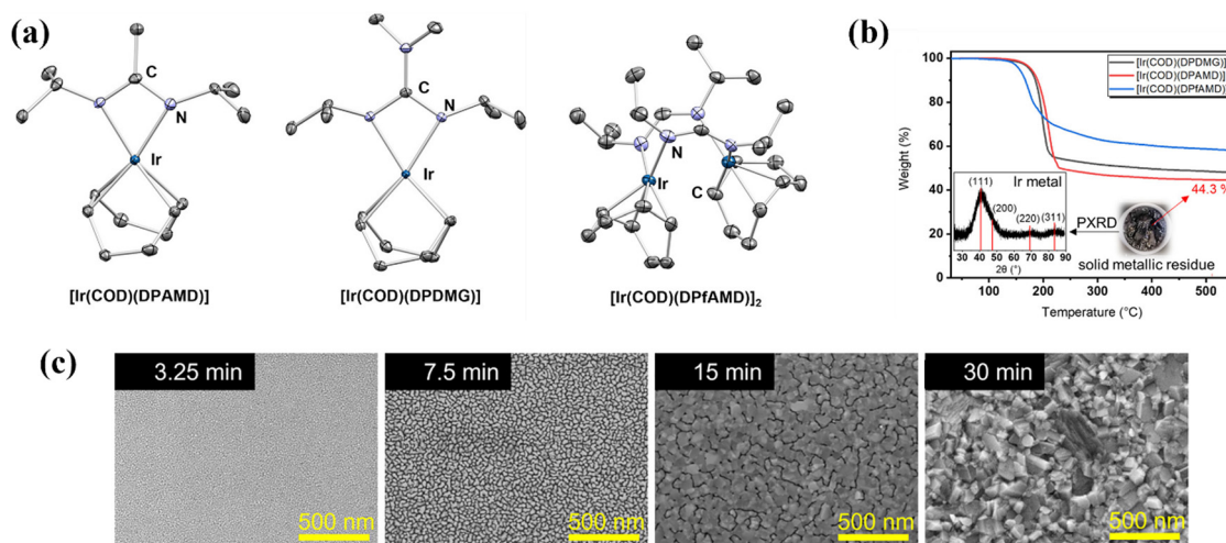
Fig. 31 (a) Structures of three bespoke Ir precursors, (b) TGA curves for the three complexes with PXR D of the residue for [Ir(COD)(DPAMD)], (c) SEM images of the Ir film deposited from [Ir(COD)(DPAMD)] with varying deposition times. Reproduced with permission from ref. 339 copyright 2022, American Chemical Society.
