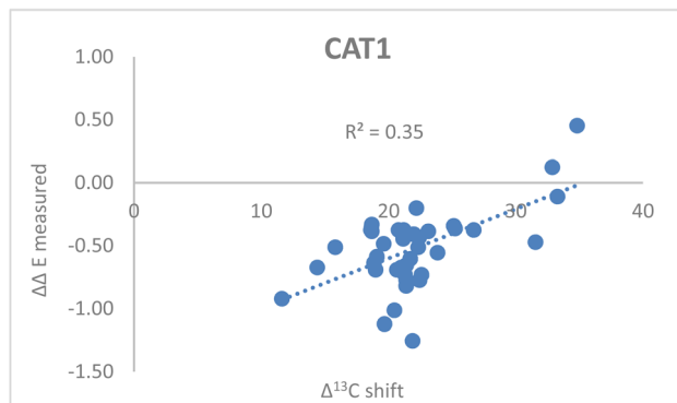
Fig. 6 Plot of the experimental regioselectivity expressed in \Delta\Delta E against the \Delta^{13}\text{C} shift for all substrates studied for the encapsulated catalyst CAT1 .
