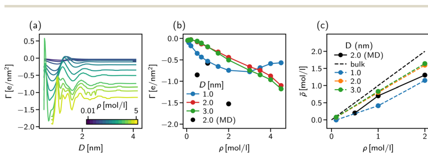
Fig. 8 Surface excess and effective concentration in solvent-explicit simulations. (a) Surface excess of ionic species in the explicit DFT model as a function of slit width. The excess is calculated with respect to the Gibbs dividing surface of the solvent species. (b) Surface excess of ionic species in the explicit DFT model as a function of bulk concentration. The three black points represent the results of the molecular dynamics simulations. (c) Effective concentration of the ionic species inside the slit as a function of bulk concentration.
