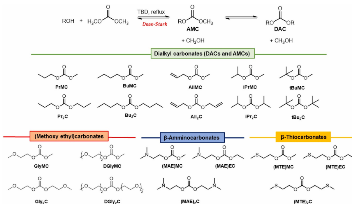
Scheme 6 Synthesis of DACs via TBD-promoted transcobonylation. Reproduced with permission from ref. 59. Copyright 2022 Elsevier Ltd.
