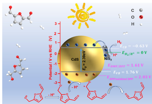
Scheme 1 Schematic illustration of the determined CB and VB edges of NiS 2 /CdS and oxidizing potential.
