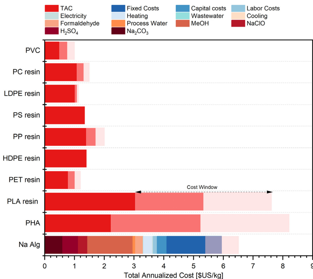
Fig. 4 TAC breakdown for NaAlg as a function of raw materials (formaldehyde, H 2 SO 4 , Na 2 CO 3 , MeOH, NaClO, process water), fixed costs, capital costs, labor costs, utilities (electricity, heating, cooling), with a direct comparison to synthetic plastic and bio-based resins. Synthetic plastics include: PVC (polyvinyl chloride), PC (polycarbonate), LDPE (low density polyethylene), PS (polystyrene), PP (polypropylene), HDPE (high density polyethylene) and PET (polyethylene terephthalate). Bio-based resins include: PLA (polylactic acid) and PHA (polyhydroxyalkanoates). Cost window signifies variability within current market prices.
