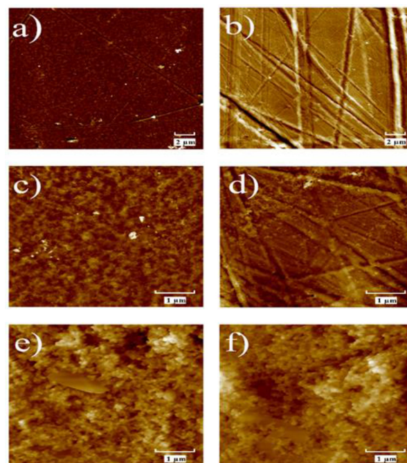
Fig. 1 Surface morphology of plastics substrate and graphite-coated screen-printed electrodes. Representative 20 \mu\text{m} \times 20 \mu\text{m} AFM images: (a) Autostat TM polyester z scale = 100 nm; (b) post-consumer PET, z scale = 100 nm. Representative 5 \mu\text{m} \times 5 \mu\text{m} AFM images: (c) Autostat TM polyester, z scale = 80 nm; (d) post-consumer PET, z scale = 50 nm; (e) SPE, z scale = 300 nm; (f) PET-SPE, z scale = 500 nm.
