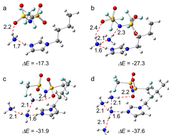
Fig. 2 The optimized structures of [BIm][Tf 2 N] with (a) one, (b) two, (c) three, and (d) four NH 3 molecules. (Color of ligand: N, blue; H, gray; C, dark gray; S, yellow; O, red; F, pale turquoise). All the distances are given in Å. \Delta E = E(\text{IL}\cdots n\text{NH}_3) - E(\text{IL}) - n \times E(\text{NH}_3) .
