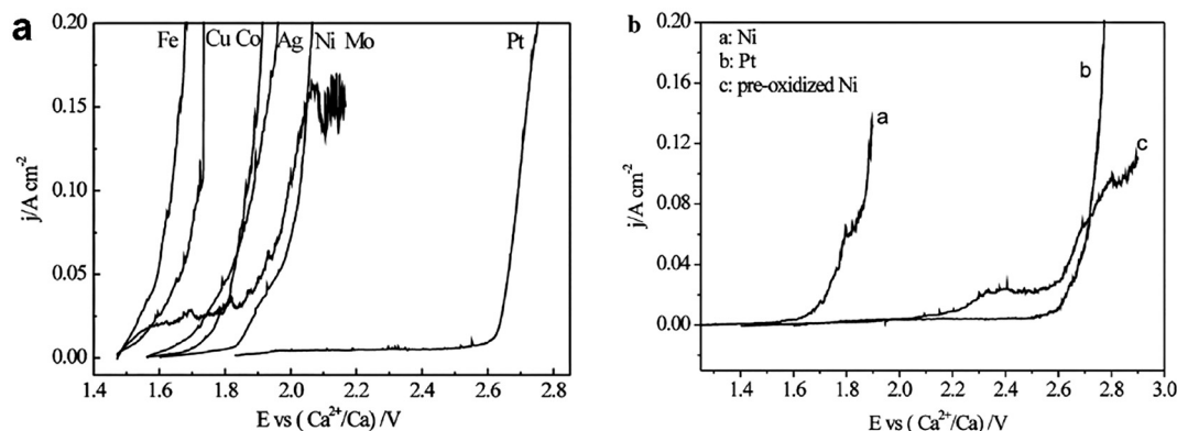
Fig. 11 (a) Polarization curves of metals in molten \text{CaCl}_2 - 2.5 \text{ mol}\% \text{ CaO} at 850^\circ\text{C} (potential scan rate, 2 \text{ mV s}^{-1} ); (b) polarization curves of Ni, Pt and pre-oxidized Ni in molten \text{CaCl}_2 at 850^\circ\text{C} (potential scan rate, 2 \text{ mV s}^{-1} ). 103
