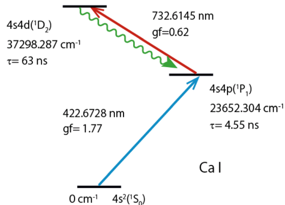
Fig. 2 Two-color two-step resonance excitation and fluorescence observation scheme of atomic Ca. Lifetimes ( \tau ) of ^1P_1 and ^1D_2 levels were cited from ref. 43,44, oscillator strengths ( gf ) of the first and second transitions from ref. 45,46, level-energies, and transition wavelengths (in air) and configurations from ref. 47,48.
