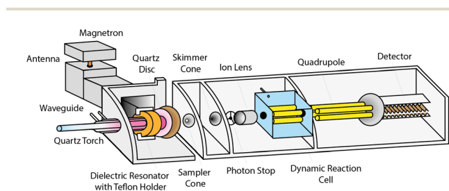
Fig. 1 Schematic depiction of the MICAP-MS.
