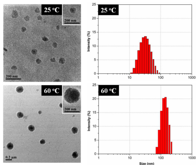
Fig. 15 TEM micrographs (left) and DLS particle size distribution by intensity (right) of micelles in copolymer solution. Reprinted with permission from ref. 289. Copyright 2012, American Chemical Society.
