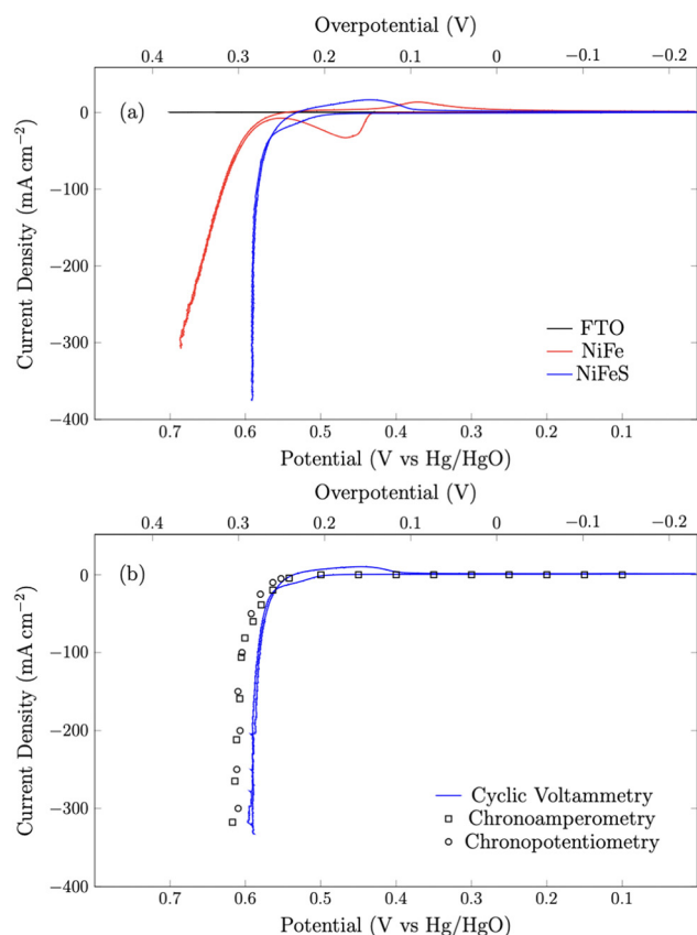
Fig. 5 (a) Cyclic voltammograms of NiFeO and NiFeS on the FTO support and blank FTO glass at a scan rate of 50 \text{ mV s}^{-1} . (b) Cyclic voltammetry data overlaid with 30-second chronoamperometry and chronopotentiometry benchmarking experiments. All experiments were performed in 3 M KOH and corrected for uncompensated resistance ( R_{\Omega} ).
