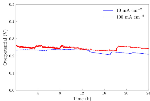
Fig. 6 Chronopotentiometry experiments on NiFeS electrodeposited FTO at current densities of 100 \text{ mA cm}^{-2} and 10 \text{ mA cm}^{-2} for 24 hours. All experiments were performed in 3 M KOH and corrected for uncompensated resistance ( R_{\Omega} ).
