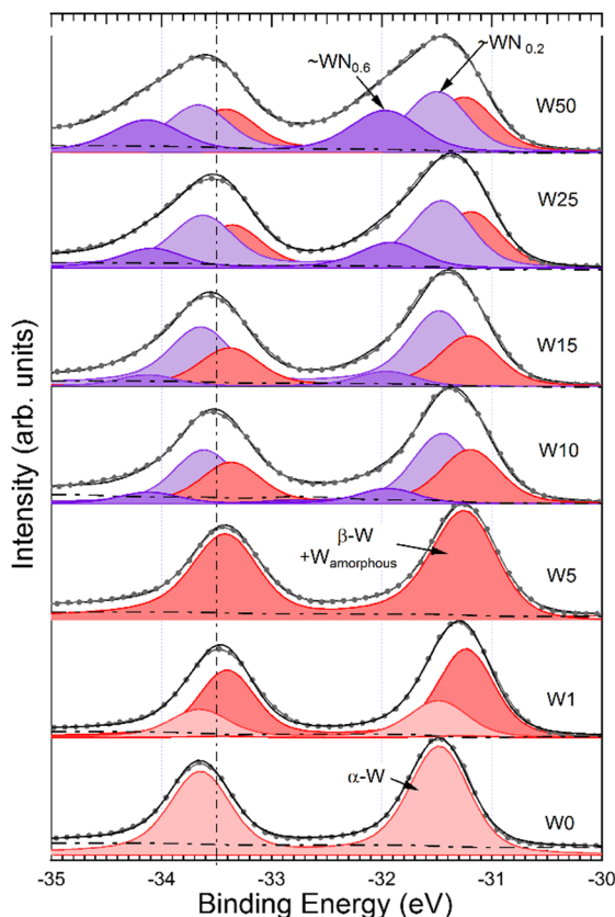
Fig. 5 W4f spectra for W thin film growth in reactive gas mixtures with N 2 (%): 0, 1, 5, 10, 15, 25, and 50. With the progressive enhancement of N 2 , we identified different W-based phases: α-W, β-W, amorphous W, WN 0.2 , and WN 0.6 .
