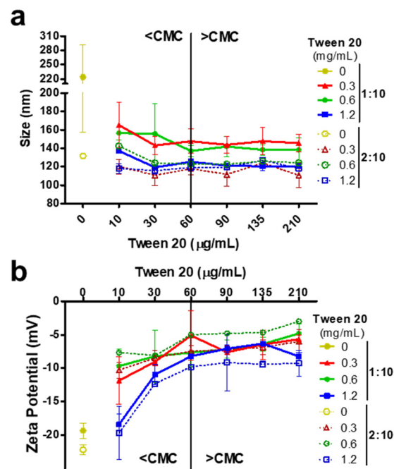
Fig. 3 Hydrodynamic diameters (a) and zeta potential (b) of CPNs characterized above and below the CMC of tween ® 20. The CPNs prepared without tween ® 20 are denoted as 0 \text{ mg mL}^{-1} .
