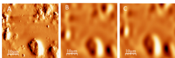
Fig. 10 AFM studies of butyl amine functionalized GO-coated Mg alloys after 5 days of immersion in 3.5% NaCl medium. (A) Butyl amine protective layer self-healing, (B) strong adsorption on the alloy surface, and (C) hydrophobic surface.
