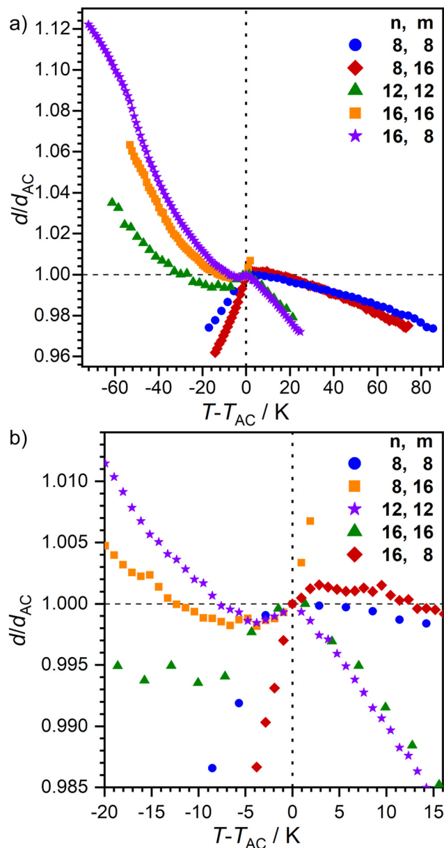
Fig. 5 Plot of the relative layer spacing d/d_{AC} as a function of T - T_{AC} for nO\text{-AzCN-PhOm} . (a) Full size and (b) close to the SmA-C transition.
