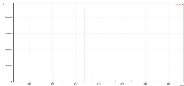
Fig. 3 ESI-MS spectra of \text{MJ}_1 [\text{M} + 1\text{H}]^+ m/z = 214.09 .
