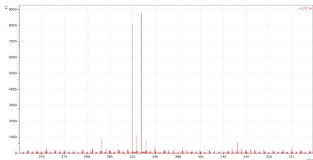
Fig. 4 ESI-MS spectra of \text{MJ}_2 [\text{M} - 1\text{H}]^- m/z = 289.98 .
