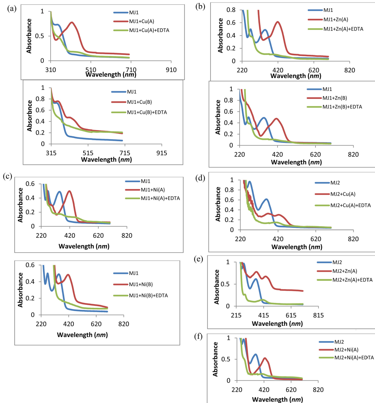
Fig. 11 (a) UV spectra of the reversibility studies of \mathbf{MJ}_1 - \text{Cu}^{2+} complexes to free \mathbf{MJ}_1 using EDTA. (b) UV spectra of the reversibility studies of \mathbf{MJ}_1 - \text{Zn}^{2+} complexes to free \mathbf{MJ}_1 using EDTA. (c) UV spectra of the reversibility studies of \mathbf{MJ}_1 - \text{Ni}^{2+} complexes to free \mathbf{MJ}_1 using EDTA. (d) UV spectra of the reversibility studies of \mathbf{MJ}_2 - \text{Cu}^{2+} complexes to free \mathbf{MJ}_2 using EDTA. (e) UV spectra of the reversibility studies of \mathbf{MJ}_2 - \text{Zn}^{2+} complexes to free \mathbf{MJ}_2 using EDTA. (f) UV spectra of the reversibility studies of \mathbf{MJ}_2 - \text{Ni}^{2+} complexes to free \mathbf{MJ}_2 using EDTA.
