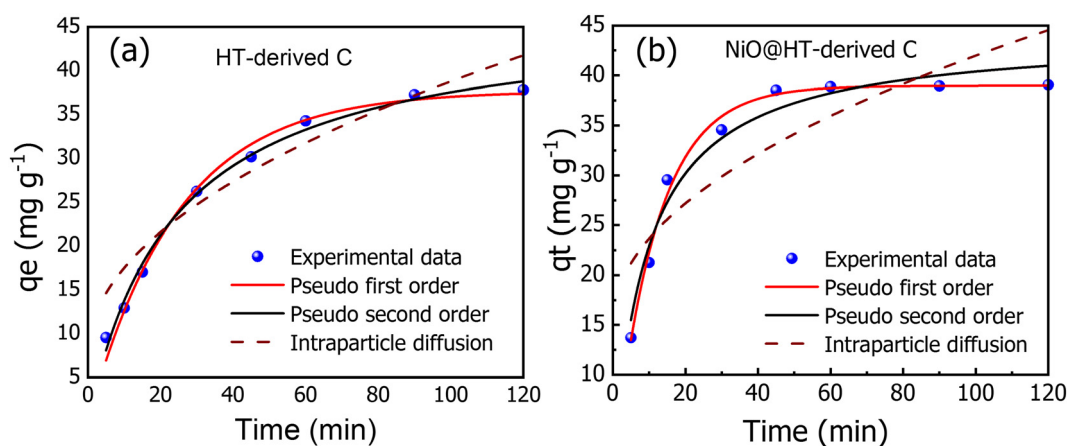
Fig. 5 The experimental and kinetic adsorption models for the adsorption of MR onto (a) HT-derived C and (b) NiO@HT-derived C adsorbents [ C_0 = 50 \text{ mg L}^{-1} , M = 0.03 \text{ g} , \text{pH} = 3 , t = 5\text{--}120 \text{ min} ].
