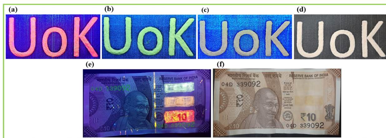
Fig. 16 Logo of the University of Kerala illuminated under UV radiation at 365 nm using security inks prepared using (a) SNMV:Eu 3+ , (b) SNMV, and (c) SNMV:Sm 3+ phosphors, and (d) under daylight, and (e) and (f) indicate the digital photographs of anti-counterfeiting labels marked on the Indian Rupee under 365 nm UV excitation (top to bottom-SNMV, SNMV:Sm 3+ and SNMV:Eu 3+ based inks) and daylight, respectively.
