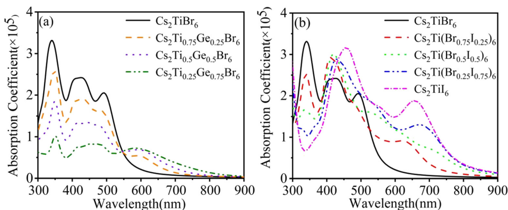
Fig. 5 Optical absorption lines. (a) \text{Cs}_2\text{Ti}_{1-x}\text{Ge}_x\text{Br}_6 ( x = 0.25, 0.5 and 0.75 ). (b) \text{Cs}_2\text{Ti}(\text{Br}_{1-x}\text{I})_6 ( x = 0.25, 0.5, 0.75 and 1 ).
