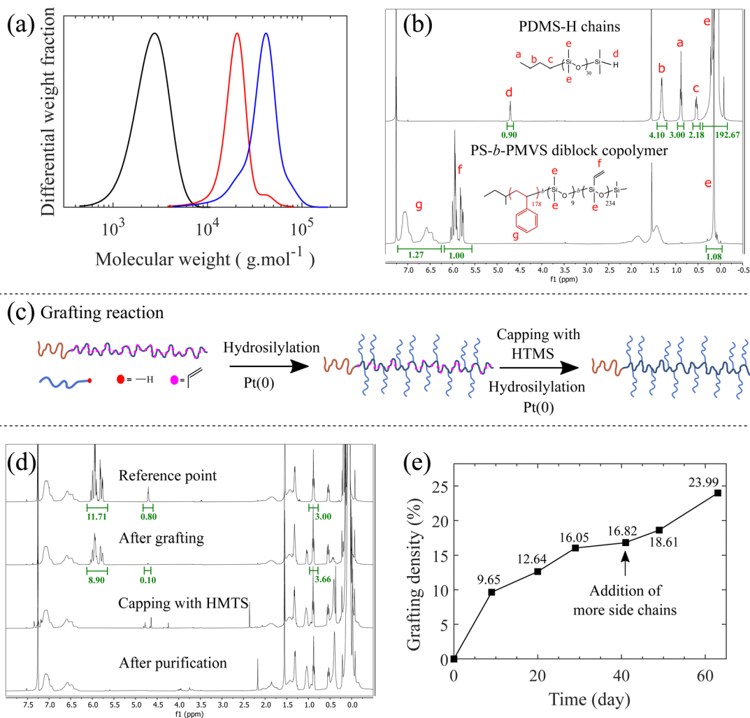
Fig. 2 Molecular characterization of synthesized materials. (a) SEC curves for the precursors of the PS- b -bbPDMS diblock copolymer. PDMS- H side chains (—) with M_n = 2260 , M_w = 2700 g mol ^{-1} , and D = 1.19 , PS block (—) in the backbone with M_n = 18\,600 , M_w = 21\,000 g mol ^{-1} , and D = 1.13 , and PS- b -PMVS diblock (—) with M_n = 33\,300 , M_w = 40\,800 g mol ^{-1} , and D = 1.22 . (b) ^1\text{H} NMR spectra of the PDMS- H (top: 400 MHz), \text{CDCl}_3 , 25 °C, \delta = 0.07 ppm (m, 3H; -Si-CH _3 ), 0.53 ppm (t, 2H, -CH _2 -), 0.88 ppm (t, 3H, -CH _3 ), 1.30 ppm (m, 4H, -CH _2 =CH _2 ), 4.70 ppm (m, 1H, -Si-H) and PS- b -PMVS diblock copolymer chains (bottom: \delta = 0.07 ppm (m, 3H; -Si-CH _3 ), \delta = 5.72 –6.10 ppm (m, 3H, -CH=CH _2 ), \delta = 6.25 –7.25 ppm (m, 5H, -C _6 H _5 )). A short block of PDMS is incorporated between PS and PMVS for the synthesis reasons to change the nature of the PS end ion to silanolate ion that ensures simultaneous propagation of living chains, as described in our previous paper. 34 (c) Schematic representation of the grafting reaction. (d) ^1\text{H} NMR spectra for the grafting reaction. The -CH _3 reference peak located at \delta = 0.88 ppm has been adjusted due to the addition of more side chains during the grafting reaction. (e) Evolution of the grafting density calculated from the consumption of the vinyl groups on the backbone.
