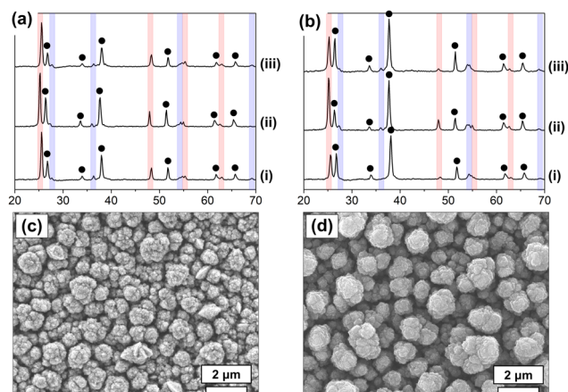
Fig. 2 (a) and (b) XRD patterns for TiO 2 films (a) (i) TiO 2 -3-80 mM, (ii) TiO 2 -3, (iii) TiO 2 -3-120 mM, (b) (i) TiO 2 -4-80 mM, (ii) TiO 2 -4, (iii) TiO 2 -4-120 mM. Peak locations corresponding to anatase and rutile phases are highlighted in red and blue respectively, and FTO is marked with a black dot. (c) and (d) Top-down electron micrographs of (c) TiO 2 -3, (d) TiO 2 -4.
