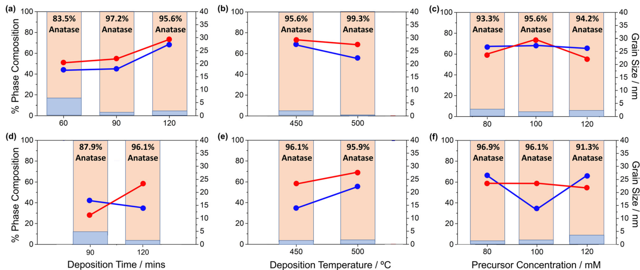
Fig. 3 Percentage compositions (bars, left axis) and crystallite grain sizes (lines, right axis) of anatase (red) and rutile (blue) in TiO 2 films deposited using (a)–(c) compound 3, (d)–(f) compound 4, as a function of (a) and (d) deposition time, (b) and (e) deposition temperature, (c) and (f) precursor concentration. Numerical anatase percent composition is shown in boxes.
