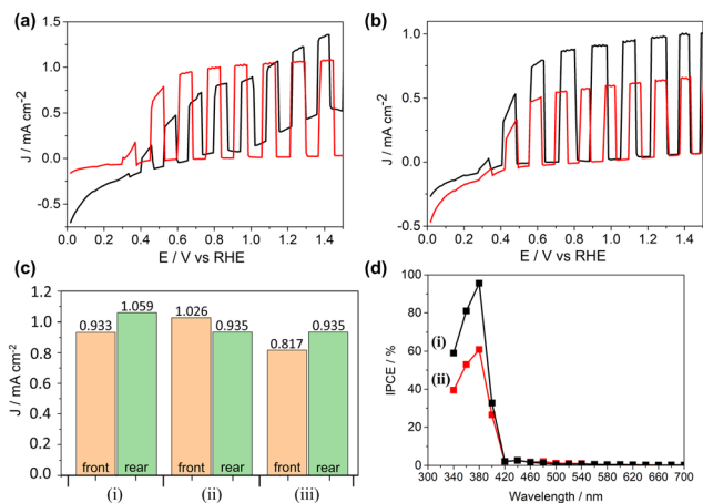
Fig. 4 (a) and (b) Linear sweep voltammograms of (a) black = TiO 2 -3, red = TiO 2 -3-80 mM, (b) black = TiO 2 -4, red = TiO 2 -4-80 mM, under 1 sun chopped AM 1.5 solar illumination; (c) Photocurrent densities at 1.23 V RHE for the highest performing TiO 2 thin films: (i) TiO 2 -3-80 mM, (ii) TiO 2 -3-60 min, (iii) TiO 2 -4; (d) incident photon-electron conversion efficiencies measured at 1.23 V vs. RHE for (i) TiO 2 -3-80 mM, (ii) TiO 2 -4. All measurements performed in 1 M KOH (pH 13.7) with a 15 mV s -1 scan rate.
