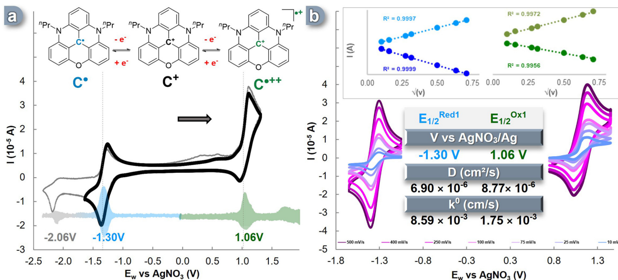
Fig. 1 (a) Three stable different oxidation states of C^+ and CV of reversible event (black) and non-reversible event (grey) at of 100 mV s -1 . DPV in reduction and oxidation in pastel color. (b) CV studies of C^+ with scan rates varying from 10 to 500 mV s -1 . Inserts show plots of anodic and cathodic peak current densities ( I ) vs. the square root of the sweep rate ( v^{1/2} ) for reduction (blue) and oxidation (green) process. Table summarizes E_{1/2} , D and k^0 obtained. Study on C^+ 1 mM in 0.1 M TBAPF 6 CH 3 CN solution, counter-anions and counter-cations have been omitted for clarity.
