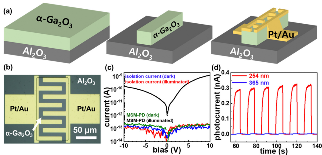
Fig. 5 (a) Schematic of the metal–semiconductor–metal photodetector (MSM PD) fabrication process. (b) The optical-microscope image of the produced PD. (c) I - V characteristics of the PD and isolated current under 254 nm UV irradiation/dark condition. (d) Time-dependent photoresponse characteristics of the fabricated MSM PD under 254 and 365 nm UV irradiations.
