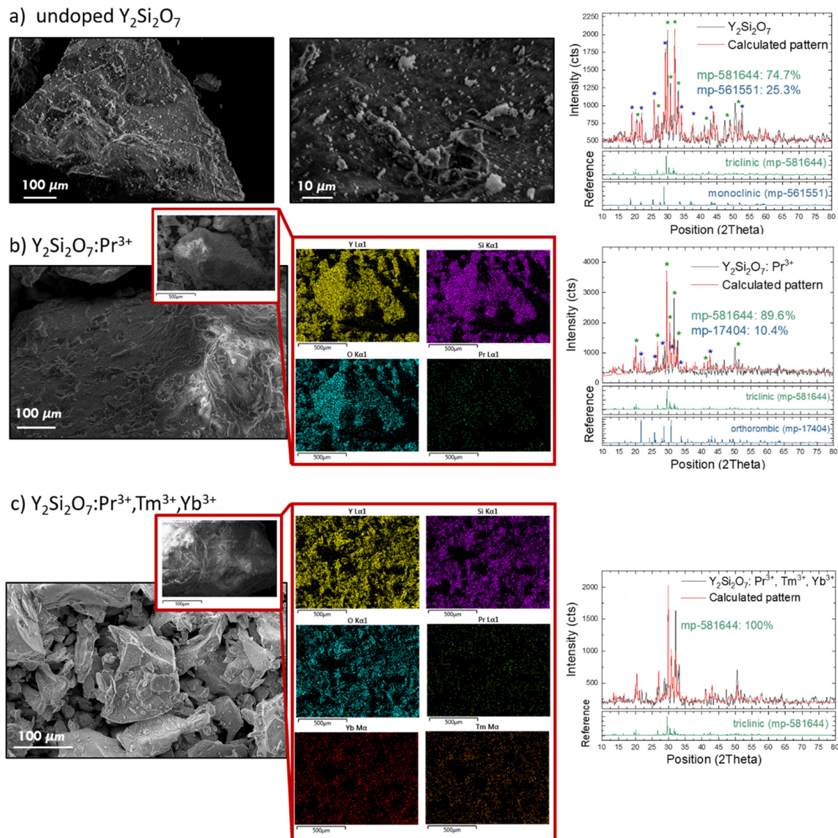
Fig. 1 Characterization of morphology – SEM images, composition – EDS maps and crystal structure – measured and calculated XRD patterns of undoped Y_2Si_2O_7 (a), Y_2Si_2O_7:Pr^{3+} (b) and Y_2Si_2O_7:Pr^{3+},Tm^{3+},Yb^{3+} powders.
