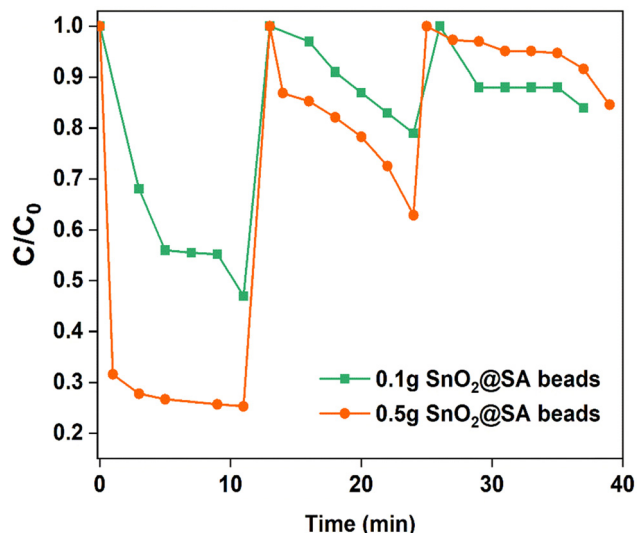
Fig. 12 Regenerative studies of 0.5 g and 0.1 g \text{SnO}_2 @SA beads for 5 \mu\text{M} CR aqueous solution.
