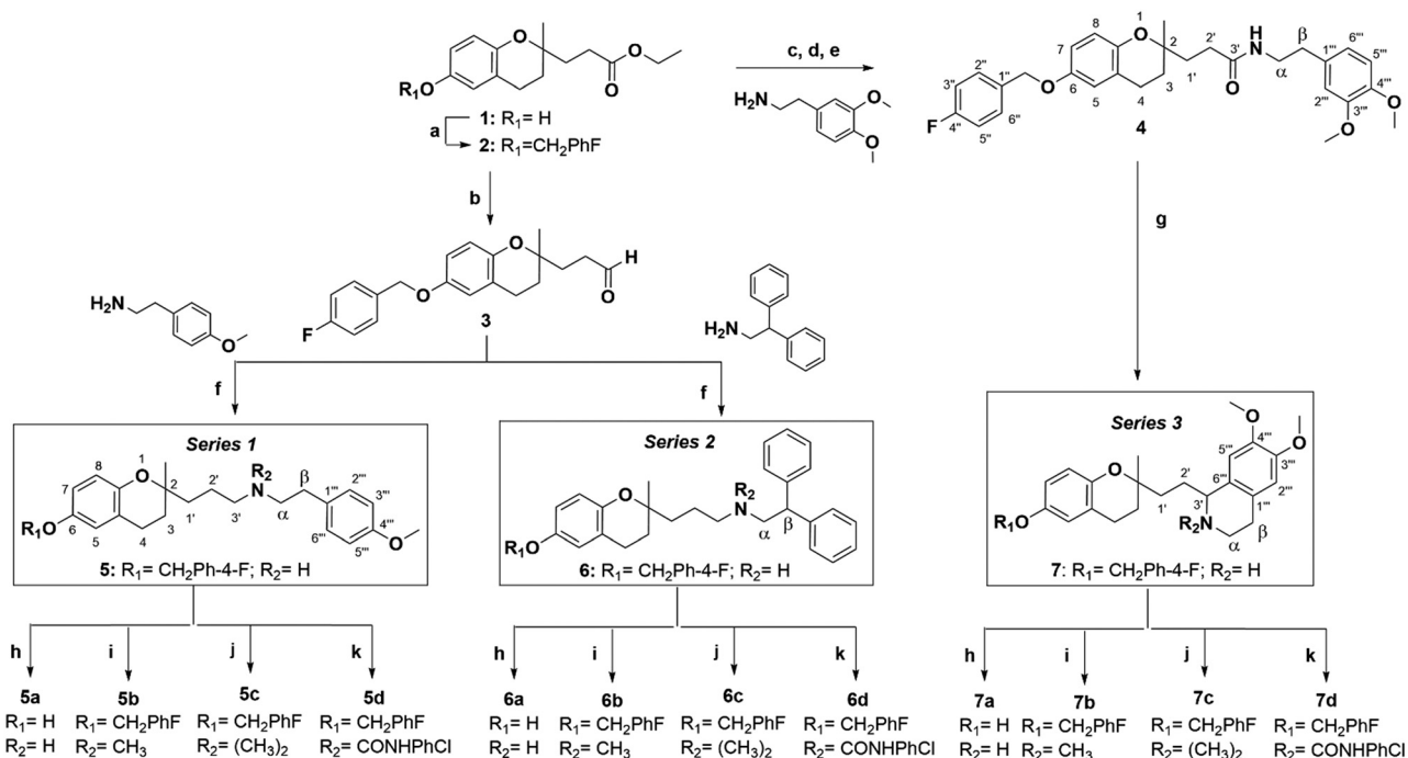
Scheme 1 Reagents and conditions: (a) p -fluorobenzyl chloride, K_2CO_3 , EtOH, reflux, N_2 , 4 h, 79%, (b) DIBAL-H, DCM, -78^\circ C , N_2 , 15 min, 92%, (c) MeOH, KOH 20%, reflux, N_2 , 4 h, (d) SOCl_2 , DCM, reflux, N_2 , 3 h, (e) 4-DMAP, Et_3N , DCM, rt., N_2 , overnight, 63%, (f) NaBH(OAc)_3 , AcOH, (CH_2Cl)_2 , rt., N_2 , 1 h, 72% for 5 and 54% for 6 , (g) POCl_3 , CH_2Cl_2 , reflux, N_2 , overnight, NaBH_4 , MeOH, rt., N_2 , 2 h, 53%, (h) HCl:EtOH 1:1, reflux, N_2 , 3 h, 92–96%, (i) HCHO , HCO_2H , MeOH, reflux, N_2 , 1 h, NaBH_4 , rt., N_2 , 45 min, 76–86%, (j) MeI, DMF, reflux, N_2 , 30 min–1 h, 79–96%, (k) 4-chlorophenyl isocyanate, Et_3N , DCM, rt., N_2 , overnight, 68–92%.
