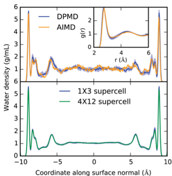
Fig. 2 Example of interfacial structure and the effect of long sampling times at the MLP level compared to short sampling at the DFT level. Top: The density profile of water confined between two TiO 2 surfaces and the oxygen radial distribution functions as obtained from DFT and from an MLP are compared. Statistics were accumulated over 40 ps. Bottom: Equivalent density profile, but this time obtained from an equilibrated 2.5 ns molecular dynamics run. Note the differences for the “second” layer, which depends strongly on the phase-space sampling and only minimally on the chosen unit-cell size. Reproduced from ref. 22.
