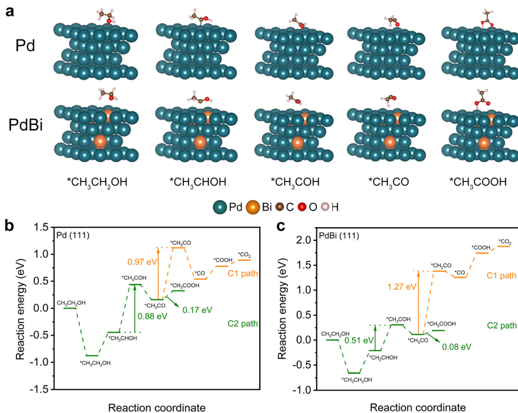
Fig. 5 Mechanistic understanding based on DFT calculations. (a) Configurations of the adsorbed intermediates for the \text{C}_2 -path of the EOR on Pd (111) and PdBi (111) slabs. (b) Calculated \text{C}_1 - and \text{C}_2 -path EOR free energy profiles on Pd (111). (c) Calculated EOR free energy profiles of \text{C}_1 - and \text{C}_2 -paths on PdBi (111).
