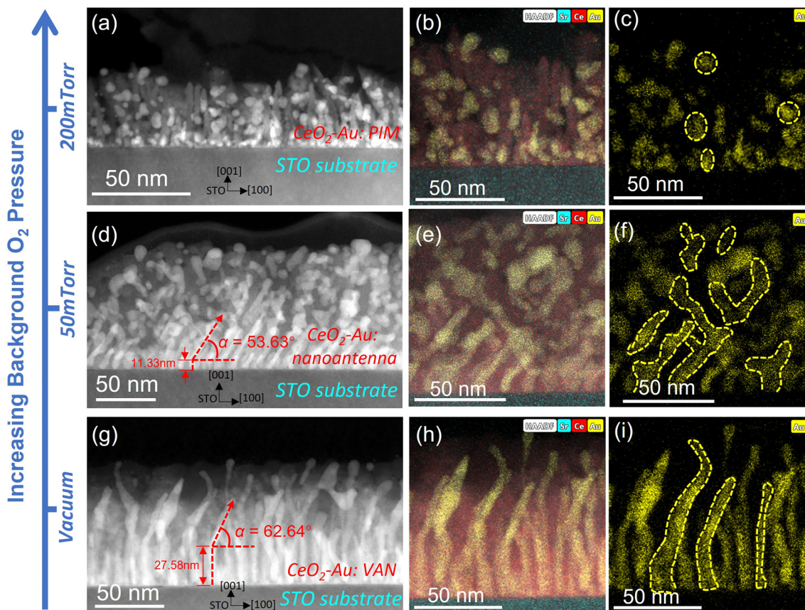
Fig. 2 STEM and EDS images showing the cross-sectional microstructure development in three sets of \text{CeO}_2\text{--Au} thin films. (a), (d) and (g) are the STEM images. (b and f) and (h and i) are the EDS images from the enlarged areas in the corresponding STEM images. (a)–(c) show the PIM sample that was deposited under 200 mTorr background oxygen pressure. (d–f) show the three-phase growth of the nanoantenna sample that was fabricated under 50 mTorr background oxygen pressure. And (g–i) shows the slightly tilted VAN growth of Au nanopillars when depositing in vacuum. In particular, the vertical growth height of Au nanopillars and tilting angles are denoted in (d) and (g).
