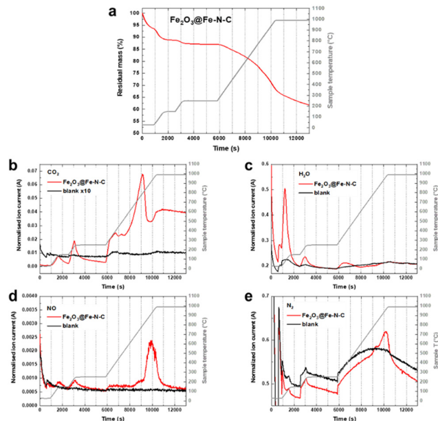
Fig. 4 (a) Results of the TGA-MS investigation of \text{Fe}_2\text{O}_3@Fe-N-C upon heating to 1000^\circ\text{C} under Ar atmosphere. TGA curve displaying the sample mass in percentage (red) and sample temperature (grey). (b) \text{CO}_2 , (c) \text{H}_2\text{O} , (d) NO and (e) \text{N}_2 MS signals for the sample (red) in comparison with a blank measurement where only the crucible without sample is employed (black). The sample temperature is displayed in grey.
