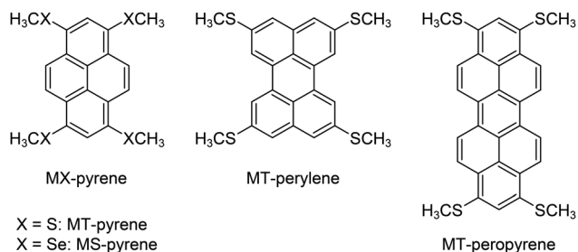
Fig. 1 Molecular structures of 1,3,6,8-tetrakis(methylthio)- and 1,3,6,8-tetrakis(methylseleno)-pyrene and (MT- and MS-pyrene), 2,5,8,11-tetrakis(methylthio)pyrene (MT-ptylene), and 1,3,8,10-tetrakis(methylthio)peropyrene (MT-peropyrene).
