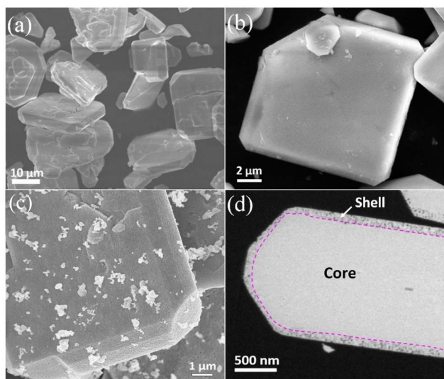
Fig. 3 SEM images of layered LaKNaNb 1-x Ta x O 5 (a) calcined at 873 K for 3 h and (b) then aged at 773 K for 15 h (c) surface and (d) cross-sectional SEM images of LaKNaNb 1-x Ta x O 5 powder nitridated at 1123 K for 4 h, revealing the porous surface.
