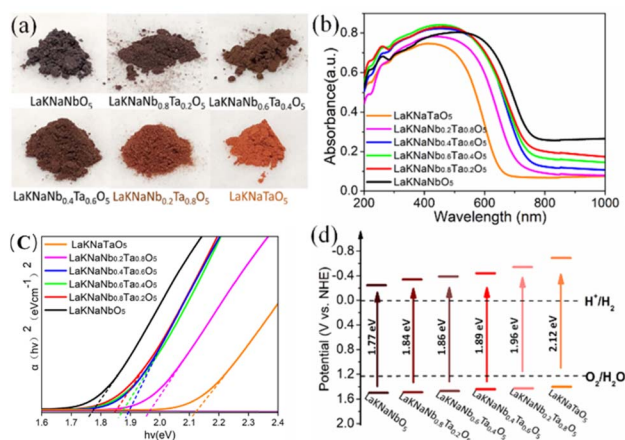
Fig. 5 (a) Photographs, (b) UV-vis DRS, (c) corresponding Tauc plots, and (d) band structure diagrams of the LaKNaNb 1-x Ta x O 5 samples ( x = 0, 0.2, 0.4, 0.6, 0.8, 1.0) nitridated at 1123 K for 4 h.
