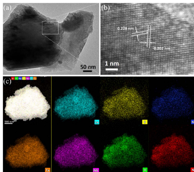
Fig. 4 (a) TEM and (b) HRTEM images and (c) EDS elemental maps of plate-like LaKNaNb 0.8 Ta 0.2 O 5 nitridated at 1123 K for 4 h. The atomic ratios were approximately La/Nb \approx 1.3, K/Nb < 0.05, Na/Nb < 0.05, O/Nb \approx 1.3, and N/Nb \approx 2.5.
