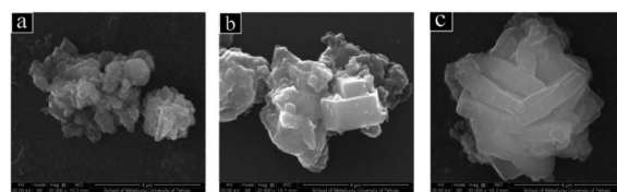
Fig. 5 SEM images of sonochemically synthesized TMU-34(-2H) after (a) 60 min, (b) 80 min, and (c) 100 min (reproduced with permission from ref. 31. Copyright 2017 Elsevier).
