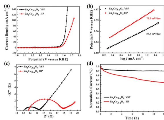
Fig. 26 (a) Linear sweep voltammetry curves and (b) Tafel plots of \text{Zn}_x\text{Co}_{3-x}\text{O}_4 YSP and \text{Zn}_x\text{Co}_{3-x}\text{O}_4 HP in an \text{O}_2 -saturated 1 \text{ M KOH} electrolyte. (c) Nyquist plots of \text{Zn}_x\text{Co}_{3-x}\text{O}_4 YSP and \text{Zn}_x\text{Co}_{3-x}\text{O}_4 HP. (d) Time-dependent current densities of \text{Zn}_x\text{Co}_{3-x}\text{O}_4 YSP and \text{Zn}_x\text{Co}_{3-x}\text{O}_4 HP (Copyright 2017, American Chemical Society). 99
