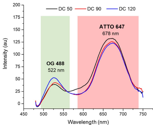
Fig. 4 Normalized fluorescence spectra of DC 50, DC 90 and DC 120 in ethanolic solution ( \lambda_{\text{ex}} = 450 \text{ nm} ).
