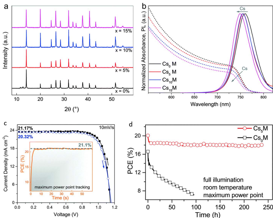
Fig. 8 Consequences of Cs accumulation in MA/FA cation blends; (a) XRD and (b) optical findings (c) current–voltage ( J – V ) and (d) stability properties of Cs x MAFA complexes (reproduced with permission from ref. 60. Copyright 2017 RSC).
