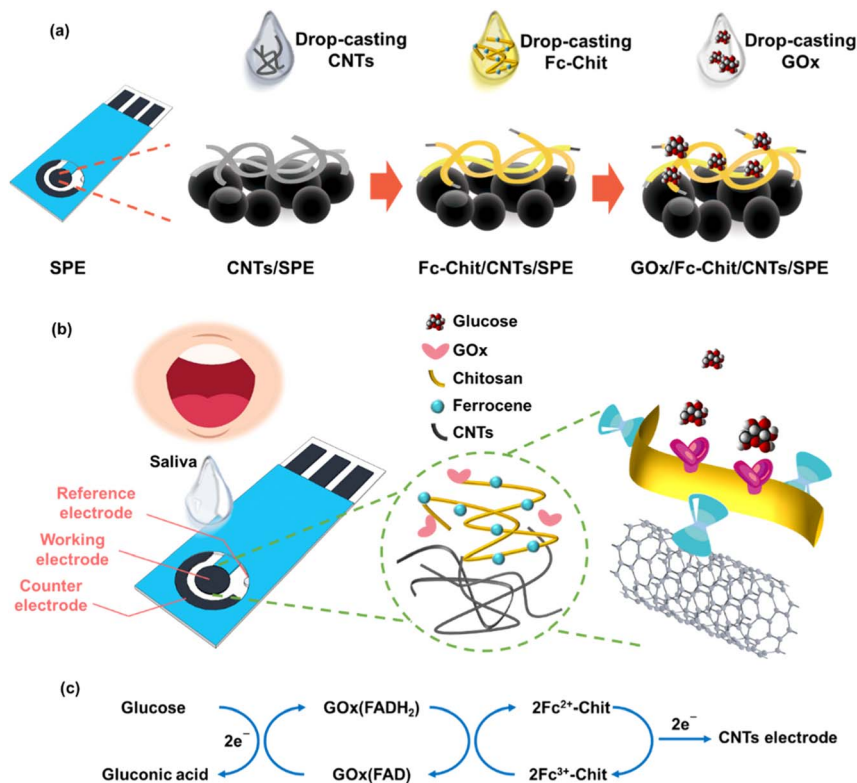
Fig. 1 Schematic illustration of the salivary glucose biosensor based on GO_x/Fc\text{-Chit}/CNTs/SPE . (a) The drop-casting fabrication sequence of the GO_x/Fc\text{-Chit}/CNTs/SPE . (b) The electrical current on the biosensor can be measured from the working to counter electrodes with Ag/AgCl as the reference electrode as it is exposed to salivary glucose. (c) For signal detection, oxidation of glucose triggered by GO_x can release electrons which can be immediately transferred to the CNT electrode by the redox Fc-Chit film.
