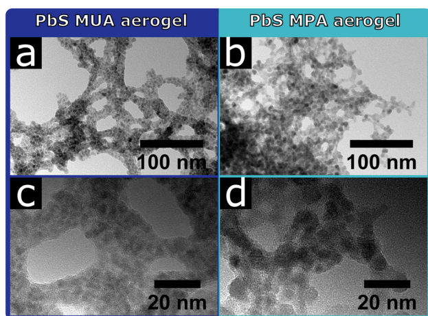
Fig. 2 The network structure of the PbS aerogels depends on the surface ligands (MUA or MPA) used during the phase transfer step. TEM images of a PbS aerogel synthesized from QDs and with YCl_3 , stabilized with (a and c) MUA, and (b and d) MPA.
