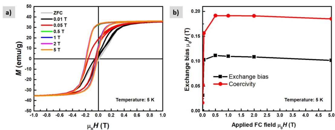
Fig. 11 M(H) loops (a) measured at 5 K temperature after field cooling in different applied magnetic fields up to \mu_0 H = 5 T. (b) Exchange bias field and coercivity as a function of the applied magnetic field during cooling.
