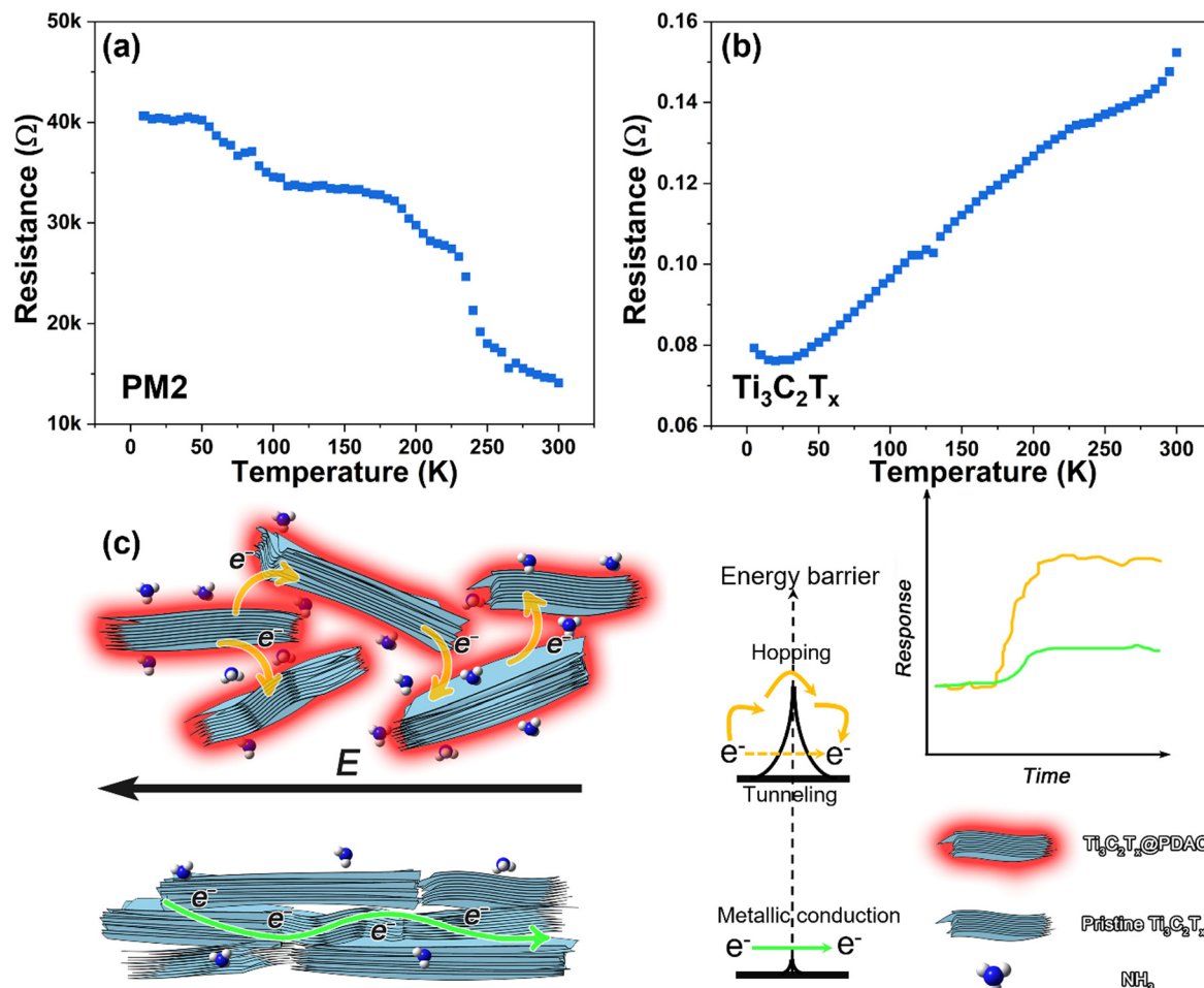
Fig. 5 Transport study and gas sensing mechanism of the Ti_3C_2T_x @PDAC composite. Temperature dependence of resistance change in (a) PM2 and (b) pristine Ti_3C_2T_x . (c) The suggested sensing mechanism of Ti_3C_2T_x @PDAC and pristine Ti_3C_2T_x .
