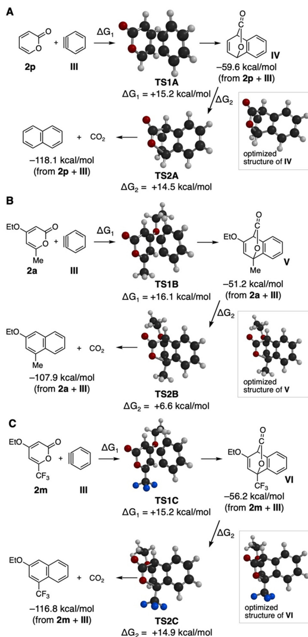
Fig. 7 (A) Calculated reaction pathways of the reaction between 2p and III . (B) Calculated reaction pathways of the reaction between 2a and III . (C) Calculated reaction pathways of the reaction between 2m and III . Atoms in TS1A–C and TS2A–C : black = C; grey = H; red = O; blue = F. See the ESI† for details.
