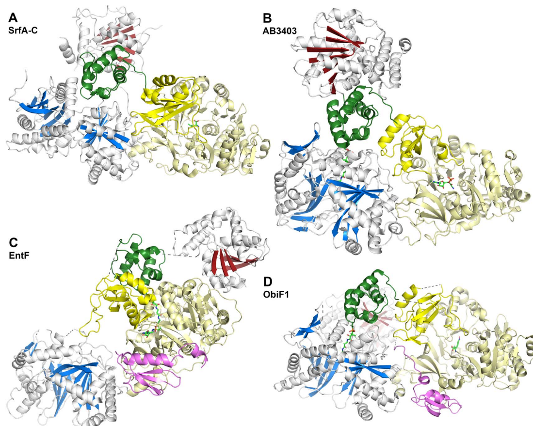
Fig. 8 NRPS termination modules. Four structures of NRPS proteins with the C-A-T-TE architecture including (A) SrfA-C (PDB 2VSQ), (B) AB3403 (PDB 4ZXI), (C) EntF (PDB 5JA1), and (D) BdObiF1 (PDB 6N8E). All structures illustrate the condensation (blue), adenylation (yellow), PCP (green) and thioesterase (red) domains. EntF and BdObiF1 also contain MLP proteins. The E. coli MLP YbdZ is bound to EntF, while the BdObiF1 contains a terminal MLP that is C-terminal to the thioesterase domain. Pantetheine and additional ligands are shown with green atoms. Note that in this orientation, the thioesterase domain of ObiF is behind the condensation domain.
