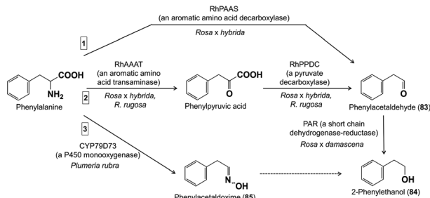
Fig. 17 2-Phenylethanol is formed by three different biosynthetic routes, and more than one may operate in a single plant species depending on the environmental conditions. The steps between phenylacetaldehyde and 2-phenylethanol are not known. Other floral volatiles are also formed by different pathways in different species or by similar pathways employing different enzymes. 52
