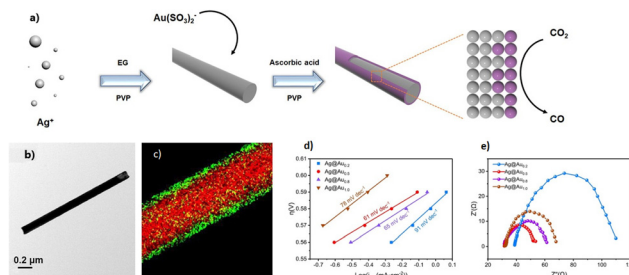
Fig. 4 (a) Schematic preparation process of Ag@Au core-shell nanowires. (b) Representative TEM image. (c) HAADF-STEM elemental mapping. (d) Tafel slope of Ag@Au 0.2 , Ag@Au 0.5 , Ag@Au 0.8 and Ag@Au 1 electrocatalysts. (e) EIS characterization of Ag@Au 0.2 , Ag@Au 0.5 , Ag@Au 0.8 and Ag@Au 1 electrocatalysts.
