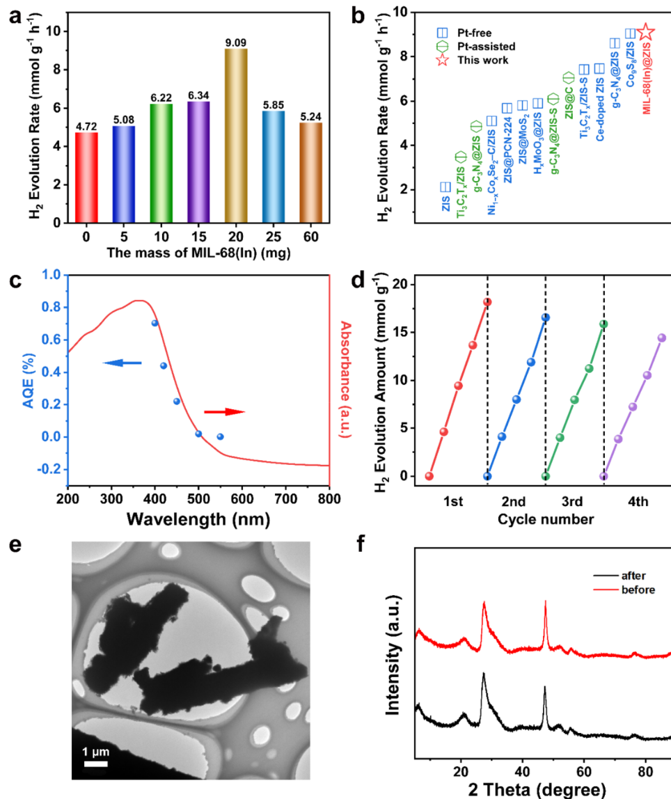
Fig. 3 Photocatalytic hydrogen production performance of photocatalysts. The photocatalytic hydrogen evolution rates of (a) MIL-68(In)- x @ZIS; (b) comparison of the hydrogen production rates of MIL-68(In)-20@ZIS in this work with those of representative photocatalysts reported recently; (c) the wavelength-dependent AQE of MIL-68(In)-20@ZIS; (d) durability test of MIL-68(In)-20@ZIS for four cycles; (e) TEM image after cycles and (f) XRD patterns before and after cycles for MIL-68(In)-20@ZIS.
