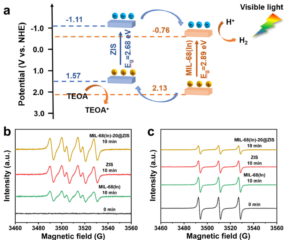
Fig. 6 The photocatalytic mechanism of MIL-68(In)@ZIS. (a) schematic illustration of charge transfer paths for MIL-68(In)@ZIS; EPR spectra of (b) DMPO ·O 2 - and (c) TEMPO h + for ZIS, MIL-68(In) and MIL-68(In)-20@ZIS.
