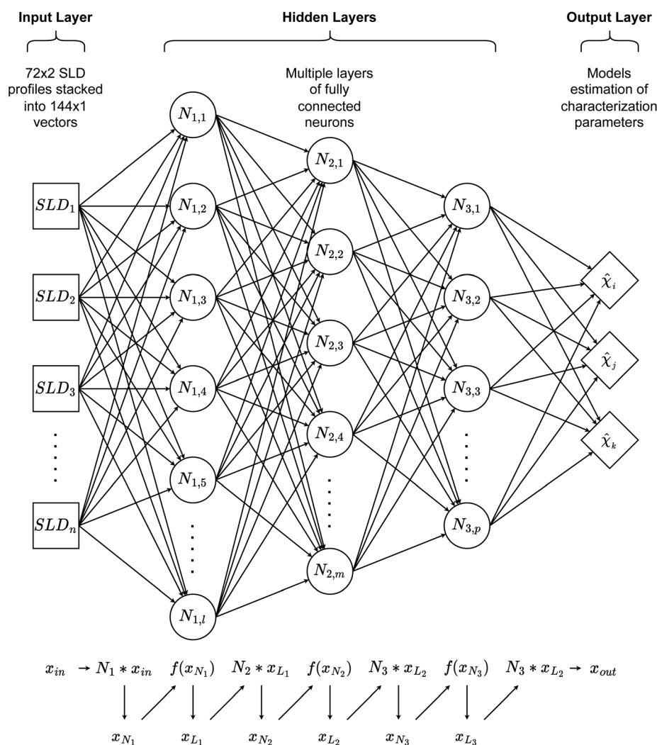
Fig. 2 Schematic representation of the multi-layer perceptron (MLP) architecture. It takes SLD curves as inputs and outputs the corresponding three Flory–Huggins parameters. Here, f(x) is an activation function.
